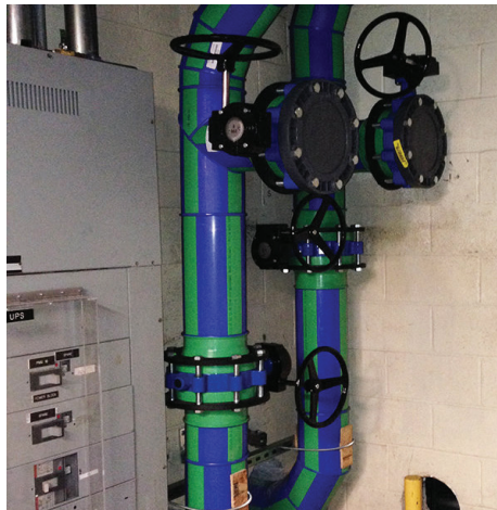
Aquatherm pipe in place during the 2014 renovation of a 1983 building into a modern data center.
