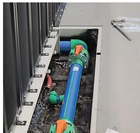
Aquatherm pipe installed (right) in a modular data center and fabricated spools in place and awaiting installation (left).
