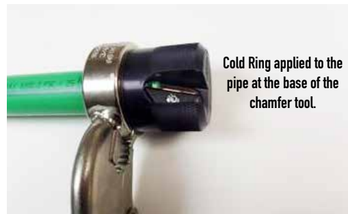
Chamfer Tool
